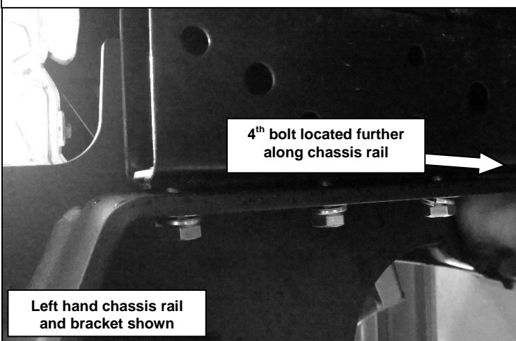
Left hand chassis rail and bracket shown
