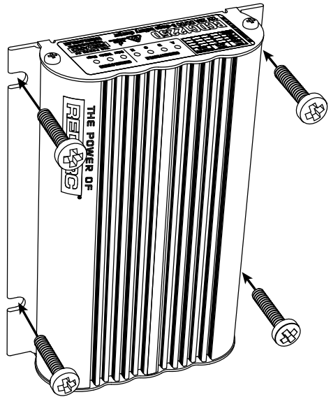
Figure 2.1.1 - Mounting the Charger
